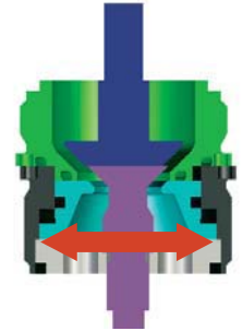
Large position tolerance (ex.: NW 13,5 mm, tolerance 2 mm)
