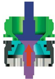
Valves in contact and media duct sealed
